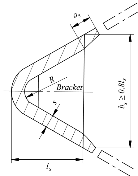
\begin{aligned} s &= 1,6s_0 \text{ for } L < 150 \text{ m}; s = 1,5s_0 \text{ for } L \geq 150 \text{ m}; \\ l_s &= 2,5L + 180 \text{ mm for } L < 200 \text{ m}; \\ l_s &= 1,4L + 400 \text{ mm for } L \geq 200 \text{ m}; \\ R &\text{— bending radius} \end{aligned}
