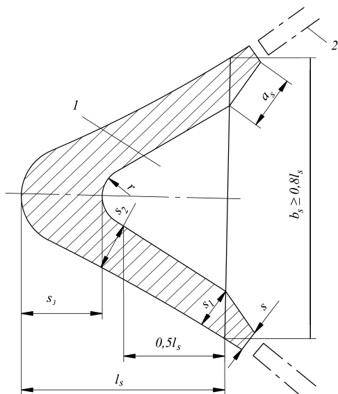
l — web; 2 — adjoining plate of shell; s_1 = 1,5s_0 ; s_2 = 2,5s_0 ; s_3 = 3,5s_0 ; l_s \geq 1,9L + 135 mm for L < 200 m; l_s \geq 1,4L + 235 mm for L \geq 200 m; r — cast radius
