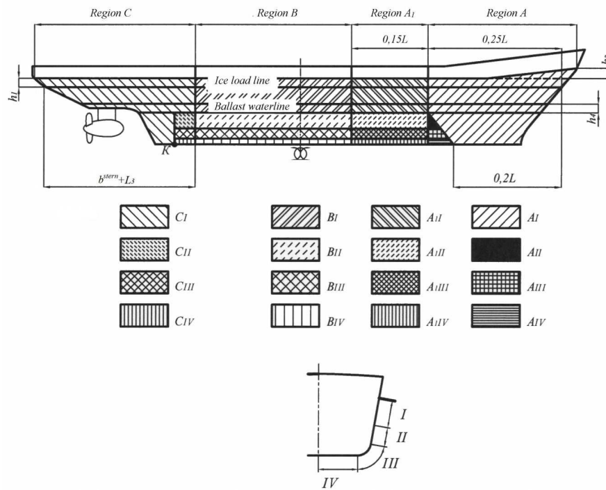
Fig. 19.2.2.4 Regions of ice strengthening of Arctic double acting ships with ice class mark Icebreaker6 or Icebreaker7 in the class notation when operating stern first:
