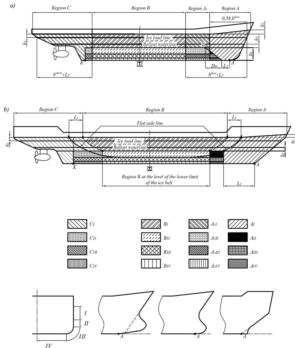
Fig. 19.2.2.3 Regions of ice strengthening of ice class ships:
