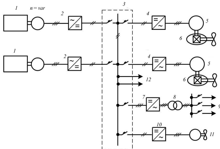
Fig. 2.2-3 Schematic diagram of PS with full distribution of the generated d.c. power with two EPP and mechanical AT:
