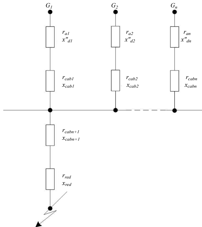
G_1 - G_n - synchronous generators; r_{a1} - r_{an} - active resistance of the generator stator winding phase at 348 K (75 °C), mOhm; x''_{d1} - x''_{dn} - sub-transient inductive resistance of the generator along a longitudinal axis, mOhm; r_{cab} - r_{cab+1} , x_{cab} - x_{cab+1} - active and inductive resistances of a.c cable segments, mOhm; r_{red} , x_{red} - active and inductive resistances of the transformer and circuit segment from rectifier leads to a SC point, as reduced to the primary winding's voltage, mOhm.
