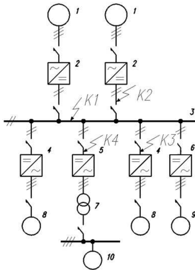
Fig. 6.1 SC design points in PS with full distribution of the generated d.c. power:
