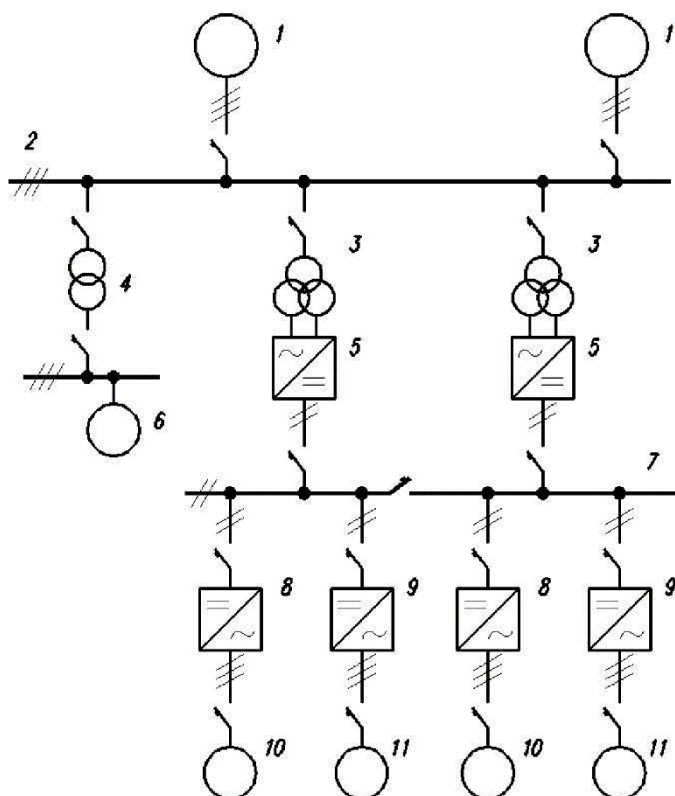
Design circuit of PS with partial distribution of the generated d.c. power:
