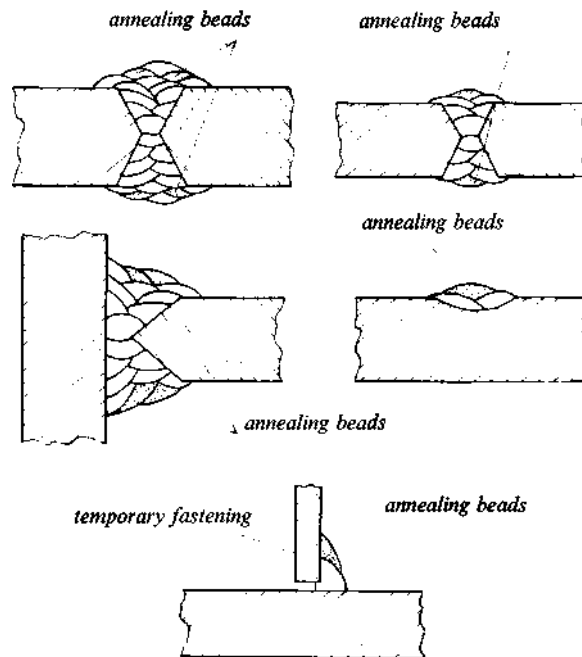
Fig. 2.8.19 Diagram showing the sequence of layers in application of "annealing beads"
