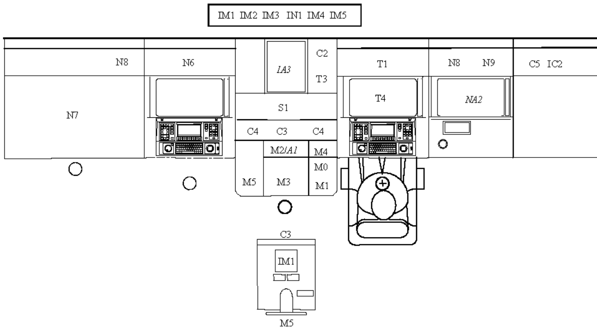
Redundant workstations
