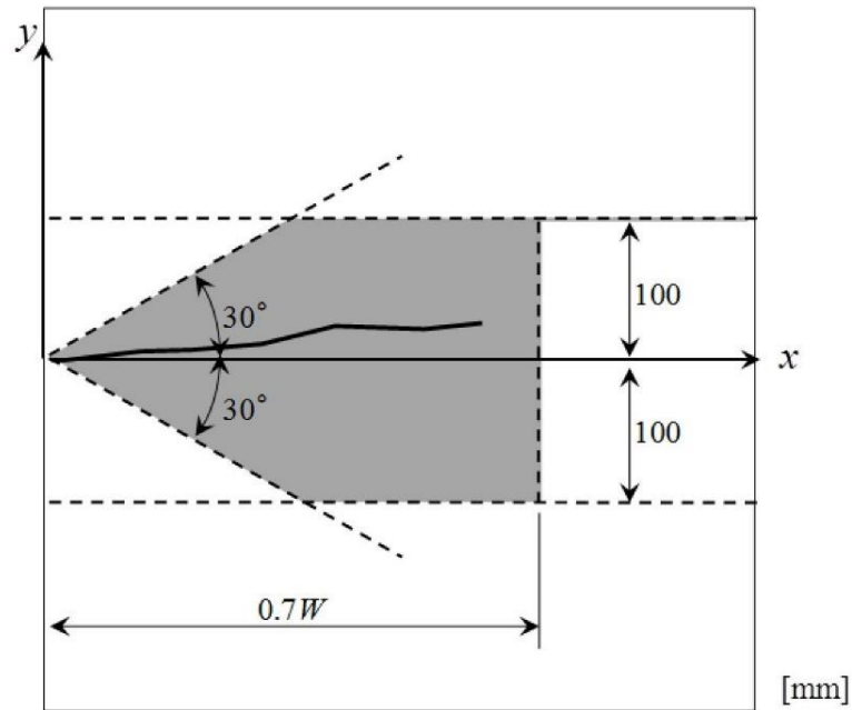
Fig. 2.2.11.1.7.1.1 Allowable range of main crack propagation path
