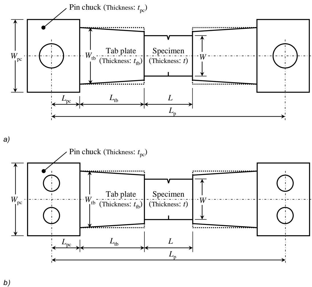
Fig. 2.2.11.1.4.2-1 Definitions of the dimensions of the tab plates and pin chucks:
