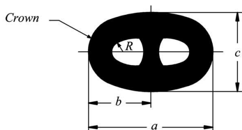
Fig. 7.2.3.2.9.2-1 Stud link — the internal link radii R and external radii shall be uniform
