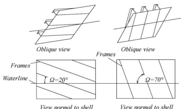
Fig. 1.2.4.2 Shell framing angle \Omega
