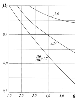
Fig. 4.2.2.8 Diagram for determining the factor \mu_T versus \varphi and HB/HB_c
