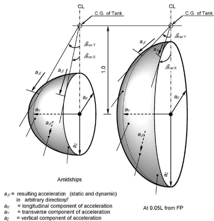
Fig. 28.1.2-1 Acceleration ellipsoid
