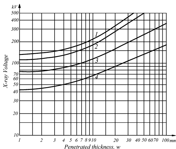
Fig. 3.2.5.5 The maximum X-ray device tube voltage values depending on the penetrated thickness of the controlled metal:
