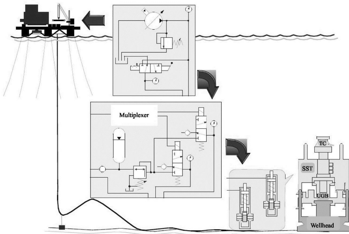
Fig. 6 Multiplex systems
