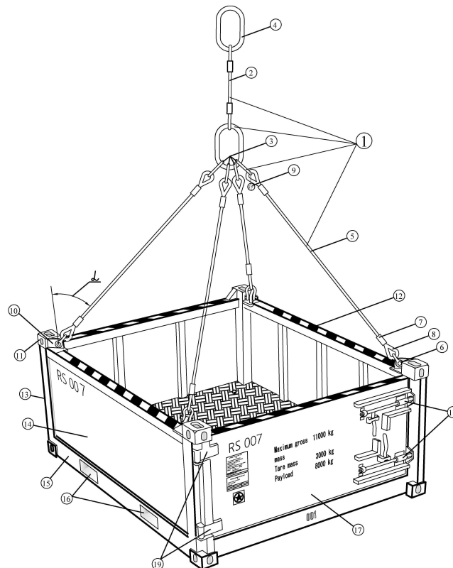
Fig. 1.2.1 Offshore container:
