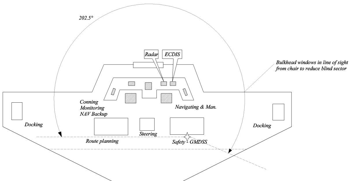
Fig. 2.5.17-2 Required field of vision from the radio station when to be controlled and infrequently used for short periods of time by the watch officer. Navigation based on electronic chart system (ECDIS) — Conning position at console
