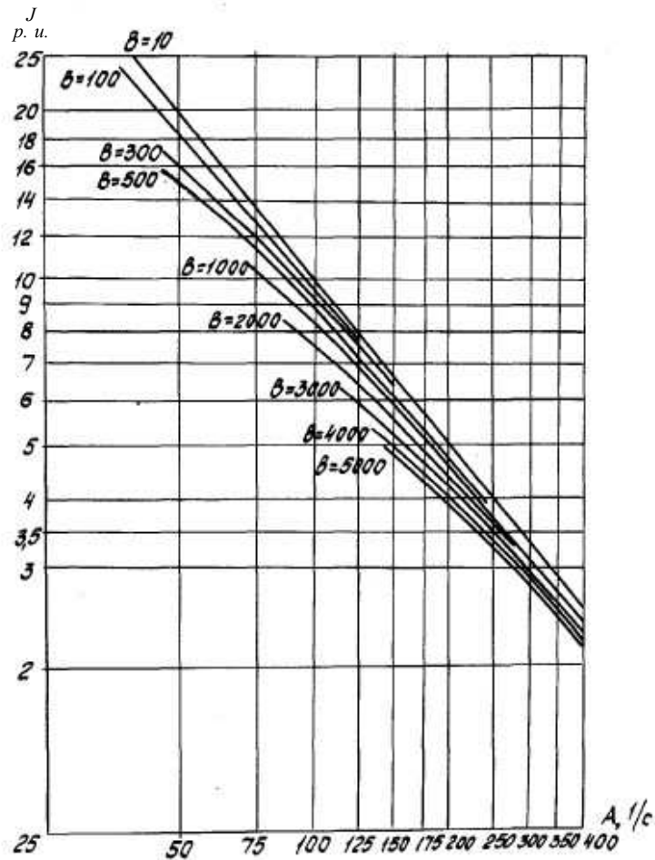
Fig. 8.4.2.2.2 Auxiliary value J as function of coefficients A and B
