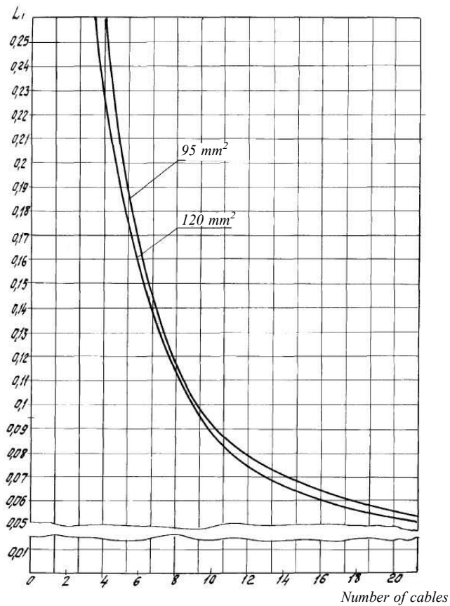
Fig. 8.6-4 Curves to determine the specific inductance of the cable run as function of the number of cables and cross-section of a conductor of cable of types "КВД-60", "КВД-100" and "КРПГ-60", H/m • 10 -6
