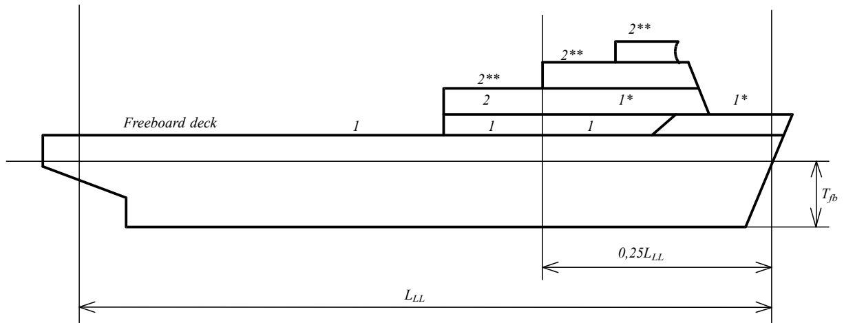
Positions 1 and 2 for an increased freeboard
