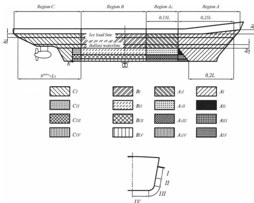
Regions of ice strengthening of Arctic double acting ships with ice class mark Icebreaker6 or Icebreaker7 in the class notation when operating stern first:
