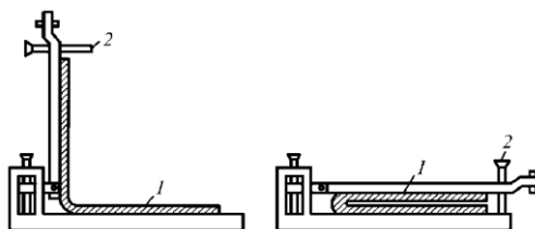
Fig. 2.3.14 Sketch of testing machine: 1 — specimen; 2 — regulating screw
