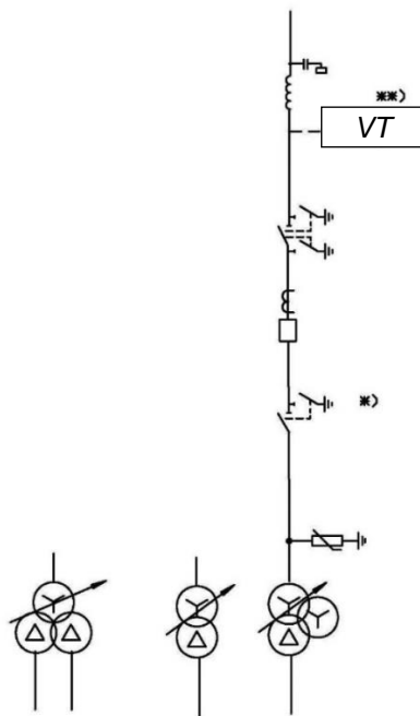
Fig. 1 unit (line — transformer) with disconnectors (diagram 110-1)
