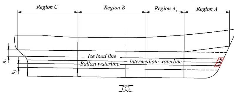
Fig. 17.7.3-1 Diagram showing control points for local deformations in region A in stem area
