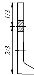
Fig. 3.2.5-4 Bulb bar
